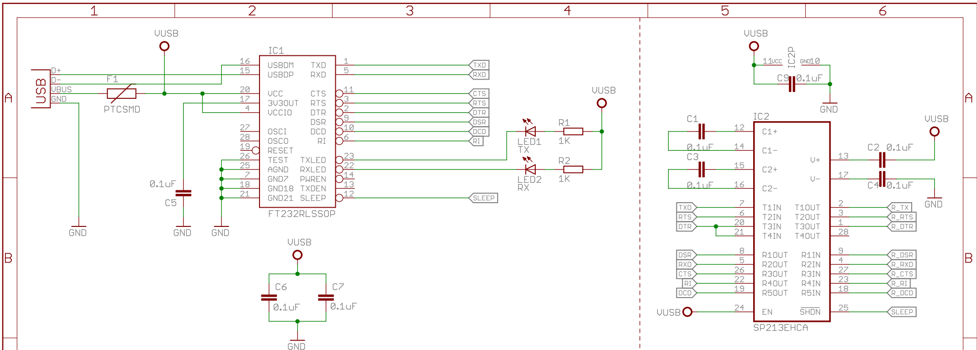
USB->Serial converter
